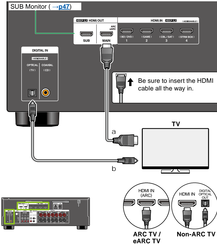
a HDMI cable, b Digital optical cable
